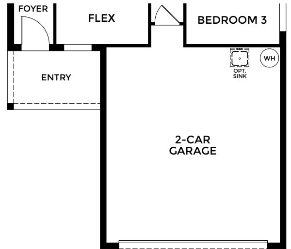
OPTIONAL 2" EXTENDED GARAGE
