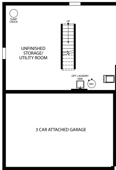
OPT. 3 CAR FRONT ENTRY GARAGE HIGH SIDE - UNFINISHED LOWER LEVEL H - ELEVATION
