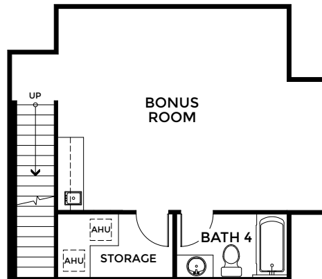
OPTIONAL BONUS BATH AND WET BAR AT ELEVATION G, H AND N
