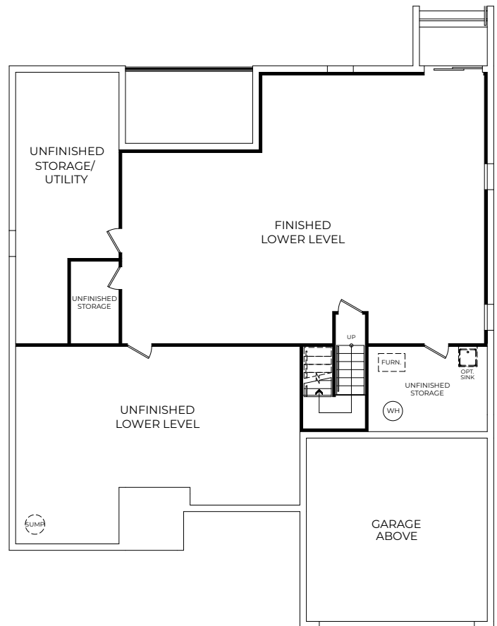
OPTIONAL FINISHED LOWER LEVEL
