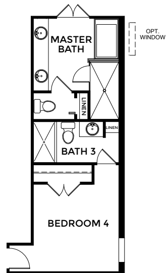
OPTIONAL DELUXE MASTER BATH W/ OPTIONAL BATH 3 AT BEDROOM 4
