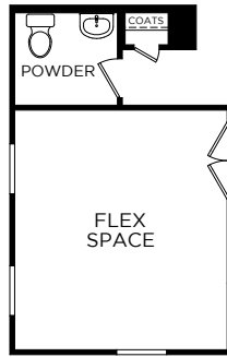
OPTIONAL DOUBLE DOORS AT FLEX
