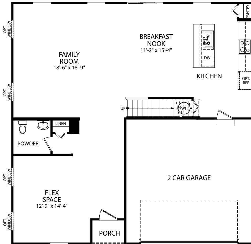
FIRST FLOOR - ELEVATION E/G
