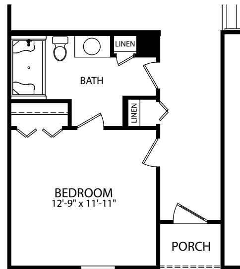
OPT. FIRST FLOOR BEDROOM & BATH
