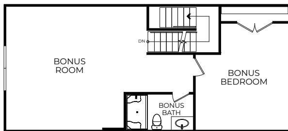
ELEVATION K SECOND FLOOR
