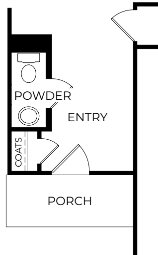
OPTIONAL POWDER ROOM
