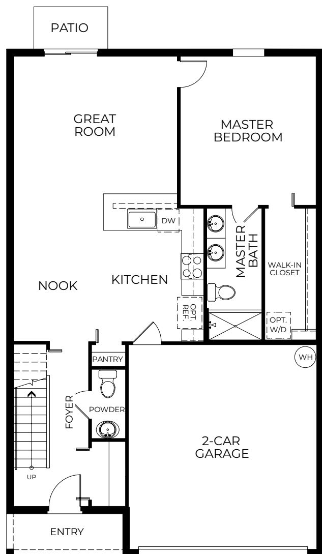
Geranium_A_Floor_1 1,024 Sq. Ft.
