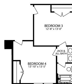
OPT. JACK & JILL BATH AT BEDROOM 3 & 4 - ELEVATION E
