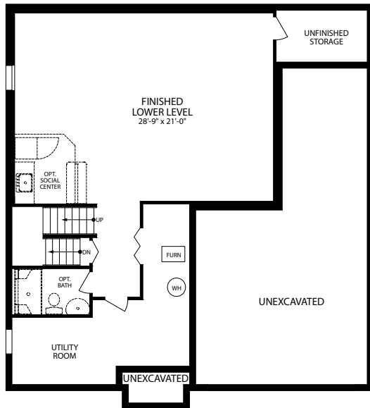
FINISHED BASEMENT
