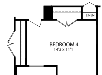
OPT. BEDROOM 4 ILO LOFT - ELEVATION K - F SERIES
