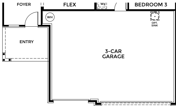
OPTIONAL 1'-4" GARAGE EXTENSION
